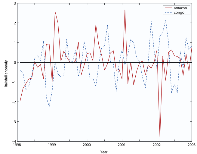
Figure 2. Rainfall anomalies over the Amazon and Congo basins. The monthly rainfall estimates for the period January 1998 to December 2002 from TRMM have been averaged over each of the two basins (Figure 1), the monthly mean removed from each series, and the resulting series of rainfall anomalies were normalized by their standard deviations. The monthly data was produced by Algorithm 3B-43 (TRMM and Other Satellites Precipitation). The purpose of Algorithm 3B-43 is to produce the “Tropical Rainfall Measuring Mission (TRMM) and Other Data” best-estimate precipitation rate and root-mean-square (RMS) precipitation-error estimates. These gridded estimates are on a calendar month temporal resolution and a 1-degree by 1-degree spatial resolution global band extending from 40 degrees south to 40 degrees north latitude. Algorithm 3B-43 is executed once per calendar month to produce the single, best-estimate precipitation rate and RMS precipitation-error estimate field (3B-43) by combining two independent precipitation fields. These two independent precipitation fields are the daily average adjusted merged-infrared (IR) estimates (3B-42) and the monthly accumulated Climate Assessment and Monitoring System (CAMS) or Global Precipitation Climatology Centre (GPCC) rain gauge analysis (3A-45). The input rain gauge data are on the calendar month temporal resolution. To obtain the requisite calendar month average of adjusted merged-IR data, 3B-43 averages the daily adjusted merged-IR data that span the calendar month of interest. After this preprocessing is complete, the two independent precipitation fields are merged together to form the best-estimate precipitation rate and RMS precipitation-error estimates. A complete description of Algorithm 3B-43 is provided in the Algorithm 3B-43 User’s Guide available from the TRMM Data and Information System (TSDIS).
