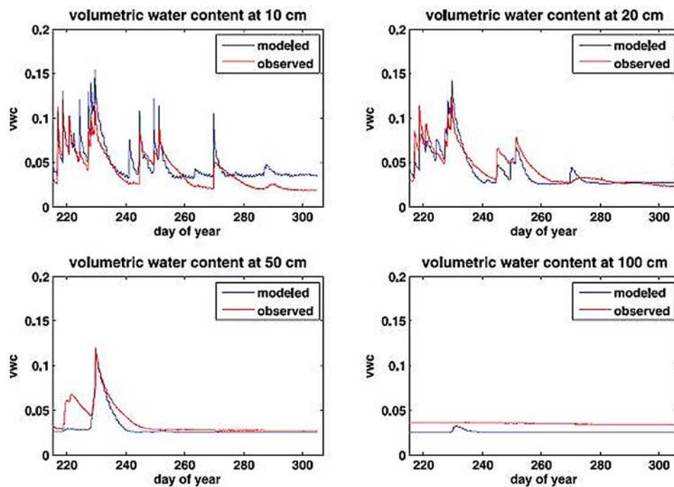
Figure 3. Model soil moisture output (volumetric water content) compared to measured soil moisture at a millet field 500 m north of Banizoumbou for the period 1 August to 10 November 2005. (Source: Bomblies et al. [2008].)
